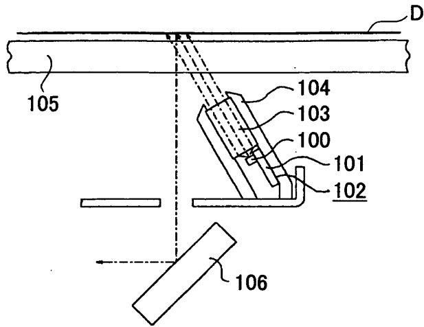
FIG.1 RELATED ART
