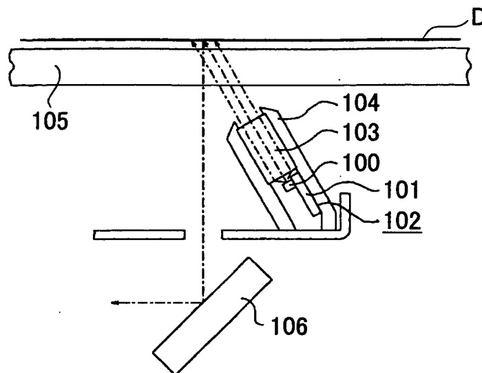
FIG.1 RELATED ART
