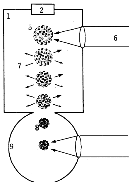
Formation of particle-cluster
