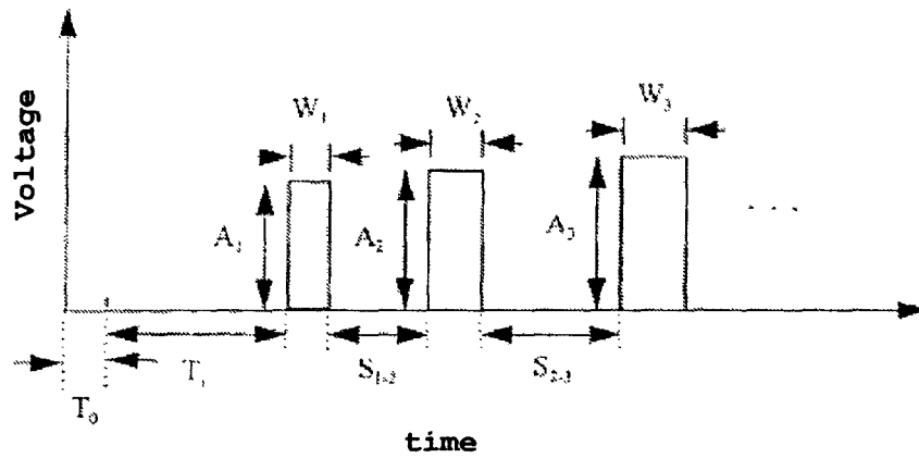
Fig. 4 - PRIOR ART
