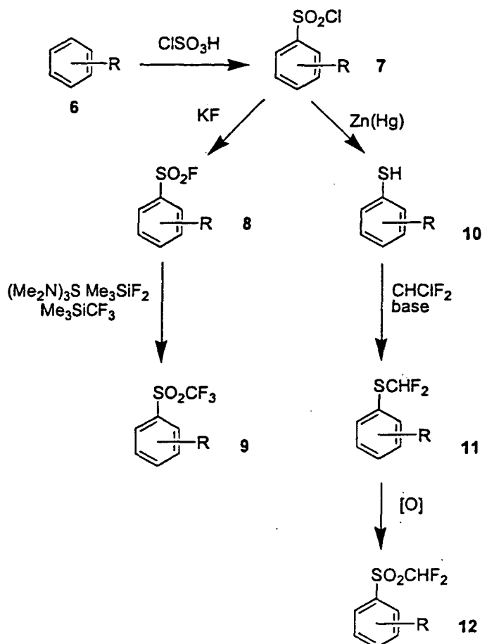
Scheme III Selected Methods of Fluorinated Aryl Sulfone Synthesis
