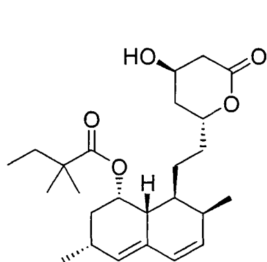
Simvastatin
