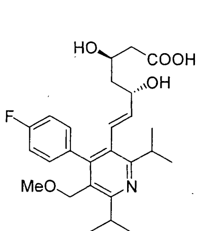
Cerivastatin
