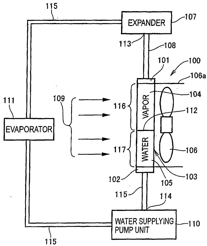
FIG. 19 (PRIOR ART)
