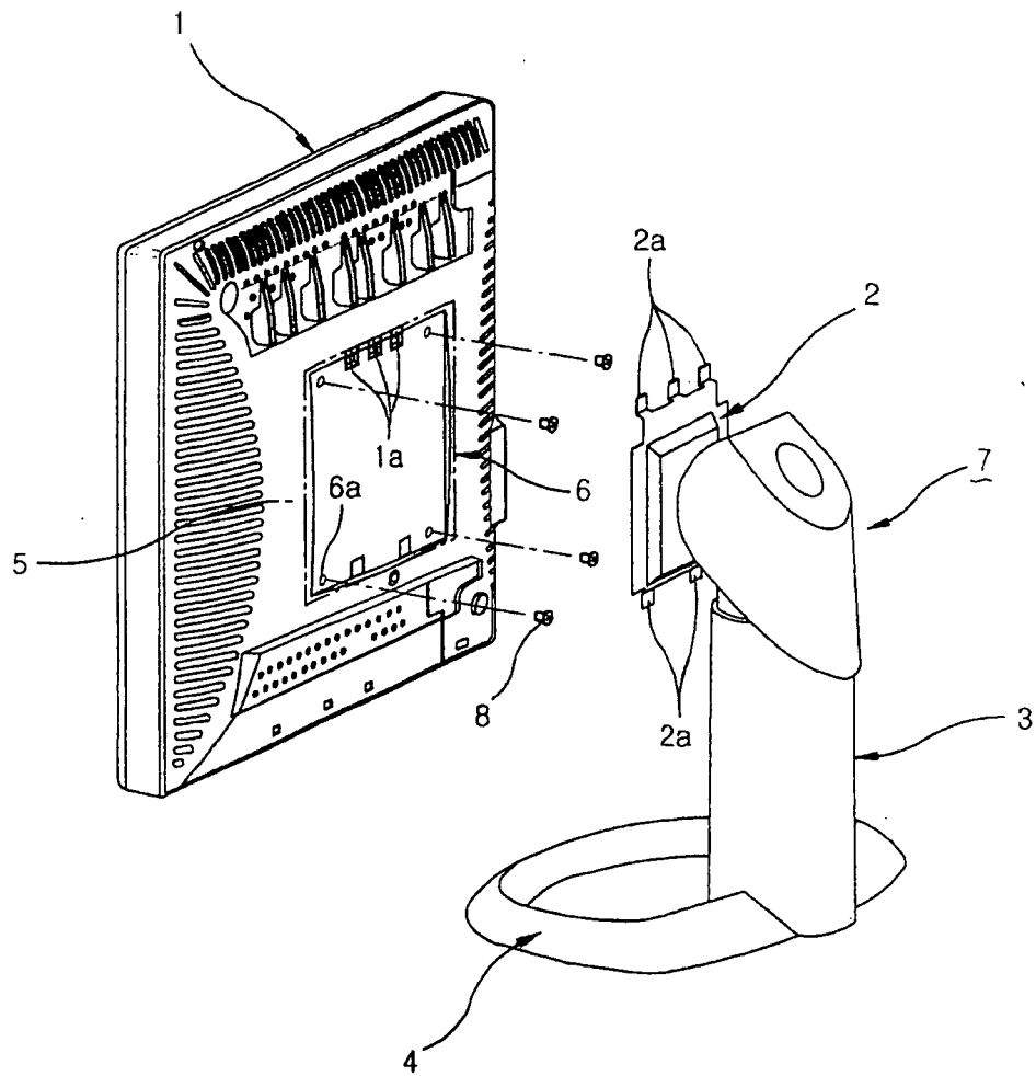
FIG. 1 RELATED ART
