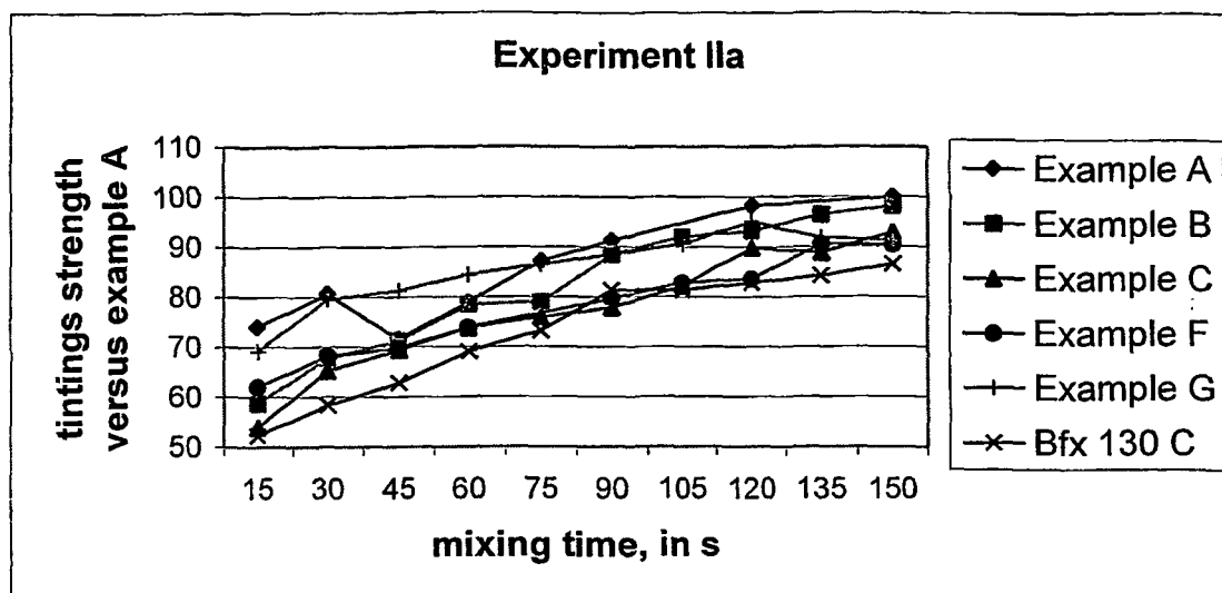
Figure 13: Development of color intensity of examples A, B,C, F, G and Bayferrox® 130 C.
