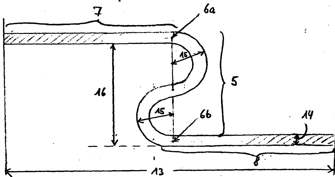
Figure 8: Seal type E
