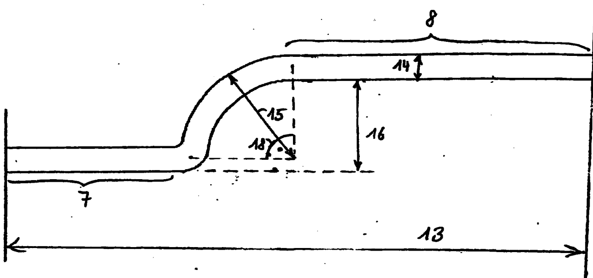
Figure 9: Seal type F
