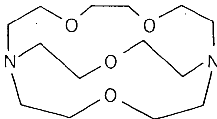
CRYPTAND [2.1.1]
