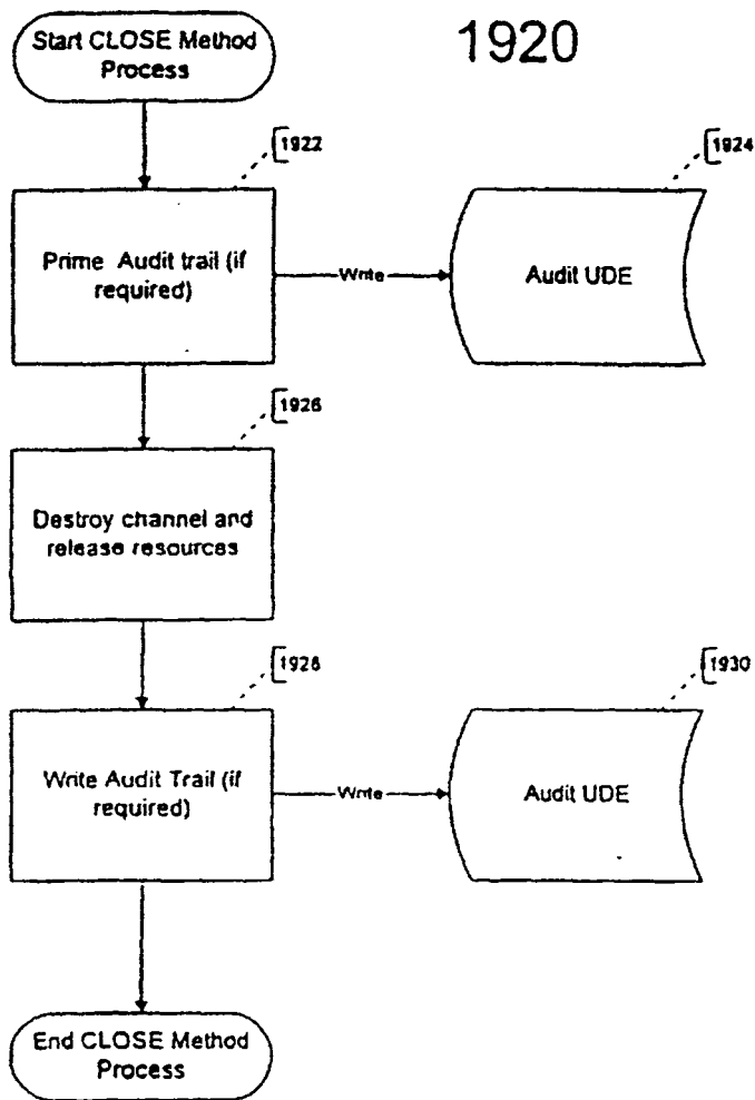
CLOSE Method Process Flow
