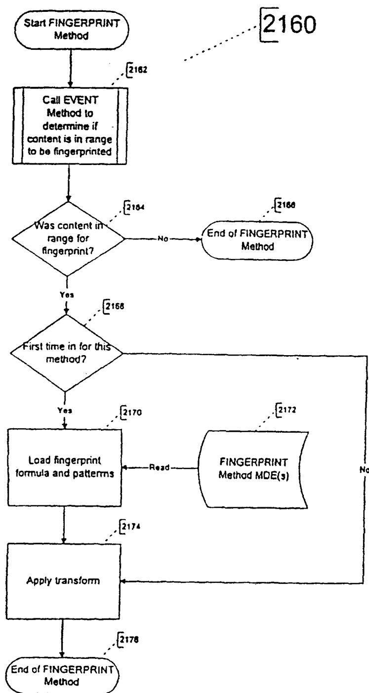
FINGERPRINT Method Process Flow
