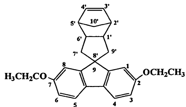
(9) Spiro[2,7-diethoxyfluorene-9,8'-tricyclo[4.3.0.12,5] [3]decene]
