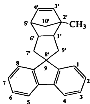
(13) Spiro[fluorene-9,8' - [2]methyltricyclo[4.3.0.12,5] [3]decene]
