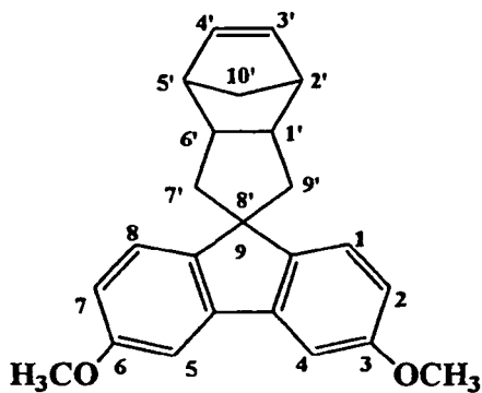
(11) Spiro[3,6-dimethoxyfluorene-9,8'-tricyclo[4.3.0.1 2,5 ][3]decene]
