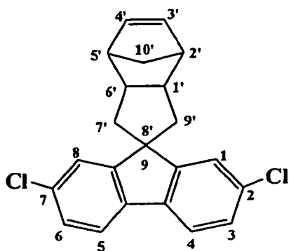
(3) Spiro[2,7-dichlorofluorene-9,8'-tricyclo[4.3.0.12,5] [3]decene]
