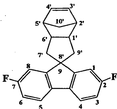
(2) Spiro[2,7-difluorofluorene-9,8' - tricyclo[4.3.0.12,5] [3]decene]
