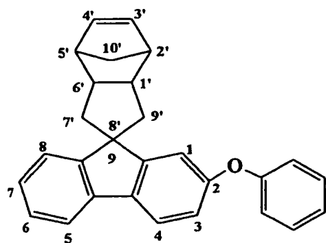
(7) Spiro[2-phenoxyfluorene-9,8'-tricyclo[4.3.0.12,5] [3]decene]
