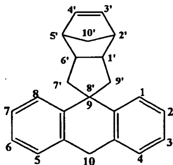
(12) Spiro[9,10-dihydroanthracene-9,8'-tricyclo[4.3.0.1 2,5 ][3]decene]
