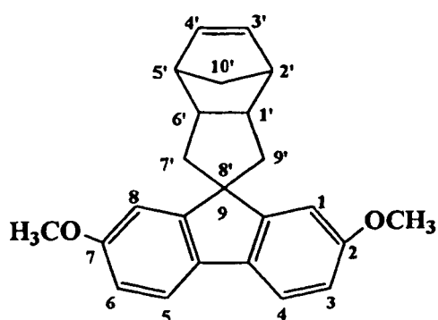
(8) Spiro[2,7-dimethoxyfluorene-9,8'-tricyclo[4.3.0.12,5] [3]decene]
