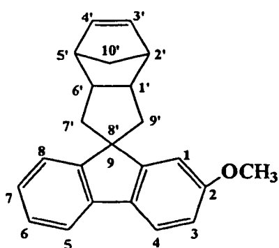
(5) Spiro[2-methoxyfluorene-9,8'-tricyclo[4.3.0.12,5] [3]decene]
