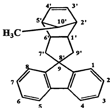
(14) Spiro[fluorene-9,8'-[10]methyltricyclo[4.3.0.12,5] [3]decene]
