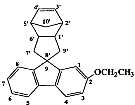
(6) Spiro[2-ethoxyfluorene-9,8'-tricyclo[4.3.0.12,5] [3]decene]
