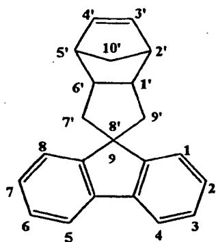
(1) Spiro[fluorene-9,8'-tricyclo[4.3.0.12,5]][3]decene]
