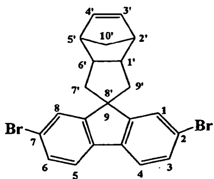
(4) Spiro[2,7-dibromofluorene-9,8'-tricyclo[4.3.0.12,5] [3]decene]
