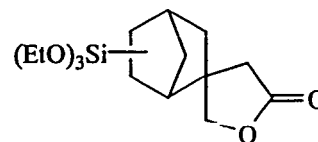
Monomer 6
