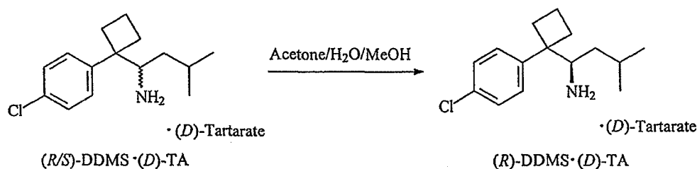
Scheme 10
