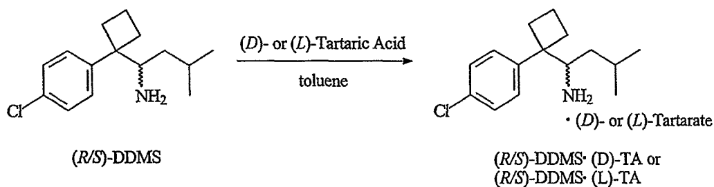
Scheme 8
