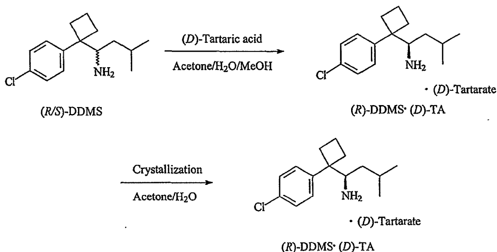
Scheme 9
