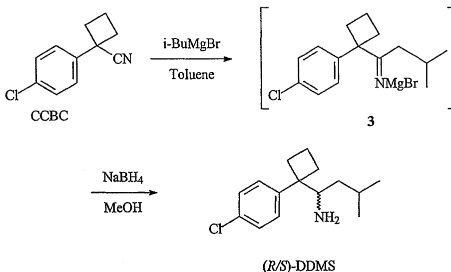
Scheme 7
