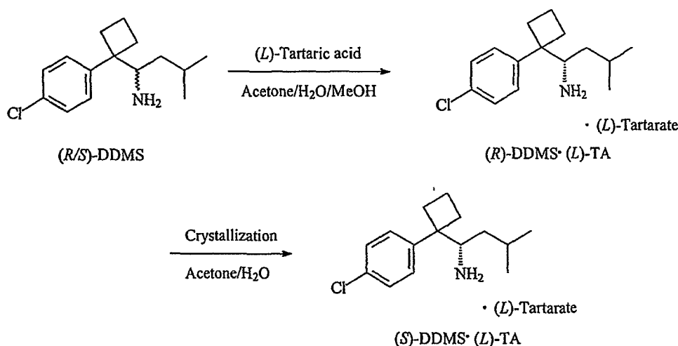
Scheme 11
