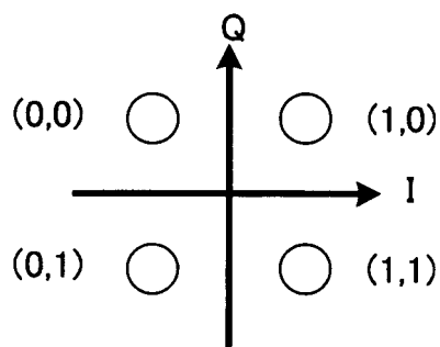
FIG. 11B S1(i)' SIGNAL POINT ARRANGEMENT
