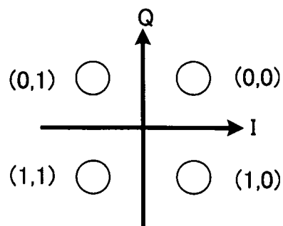
FIG.3A S1(i) SIGNAL POINT ARRANGEMENT
