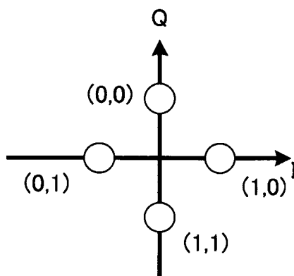
FIG. 11C S1(i)'' SIGNAL POINT ARRANGEMENT
