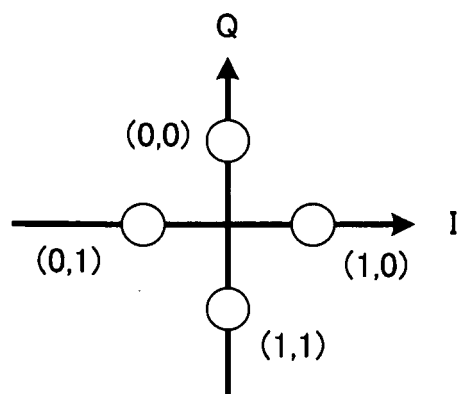
FIG.3C S1(i)' SIGNAL POINT ARRANGEMENT
