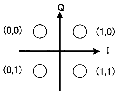
FIG.3B S1(i)' SIGNAL POINT ARRANGEMENT
