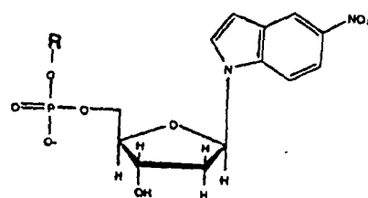
5-nitroindole
