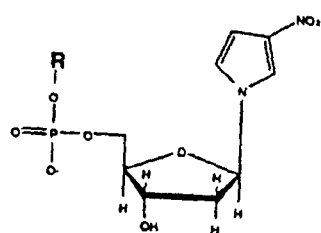
3-nitropyrrole
