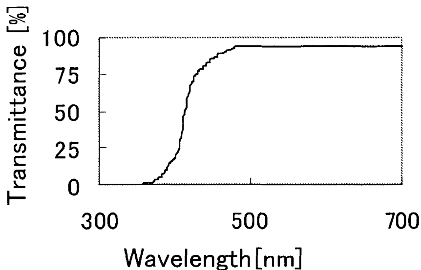
Fig.2 Transmission spectrum of the polyimide silicone in Preparation Example 5
