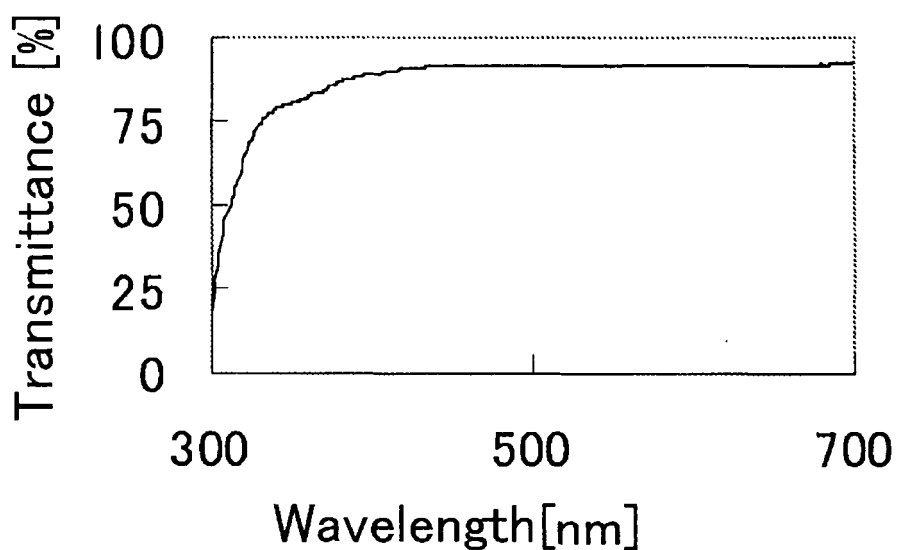
Fig.1 Transmission spectrum of the polyimide silicone of Preparation Example 1
