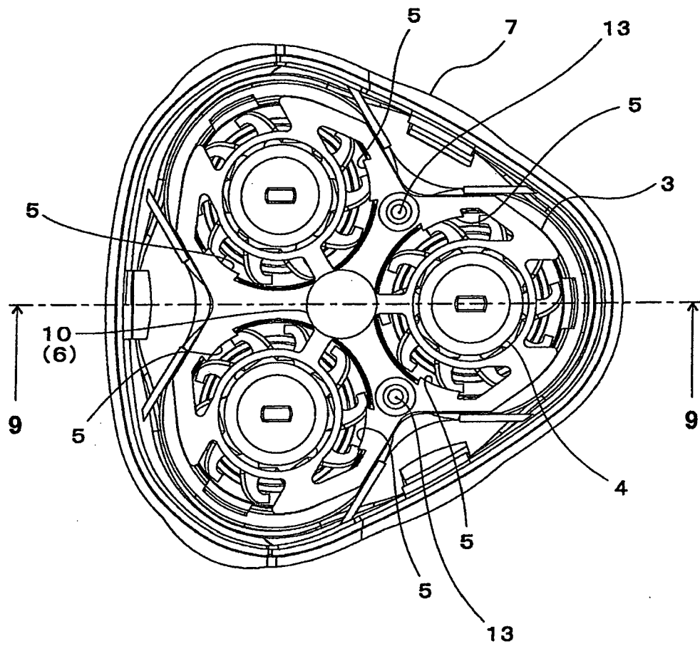
FIG. 8 PRIOR ART
