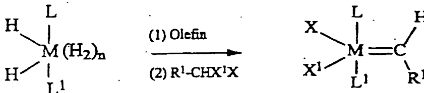
REACTION SCHEME 1
