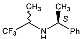
[Chem. 10]
