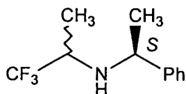
[Chem. 8]
