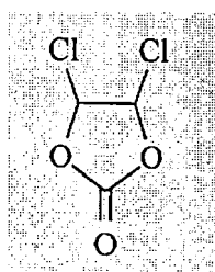
[Chemical Formula 6]
