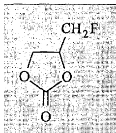
[Chemical Formula 9]
