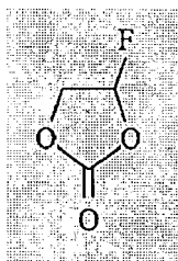
[Chemical Formula 1]
