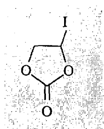
[Chemical Formula 8]
