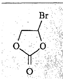
[Chemical Formula 7]
