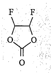
[Chemical Formula 3]
