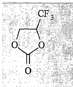
[Chemical Formula 10]
