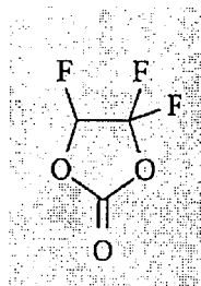
[Chemical Formula 4]
