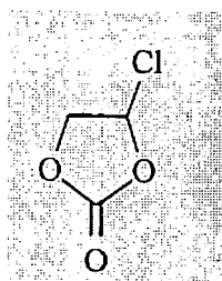
[Chemical Formula 5]
