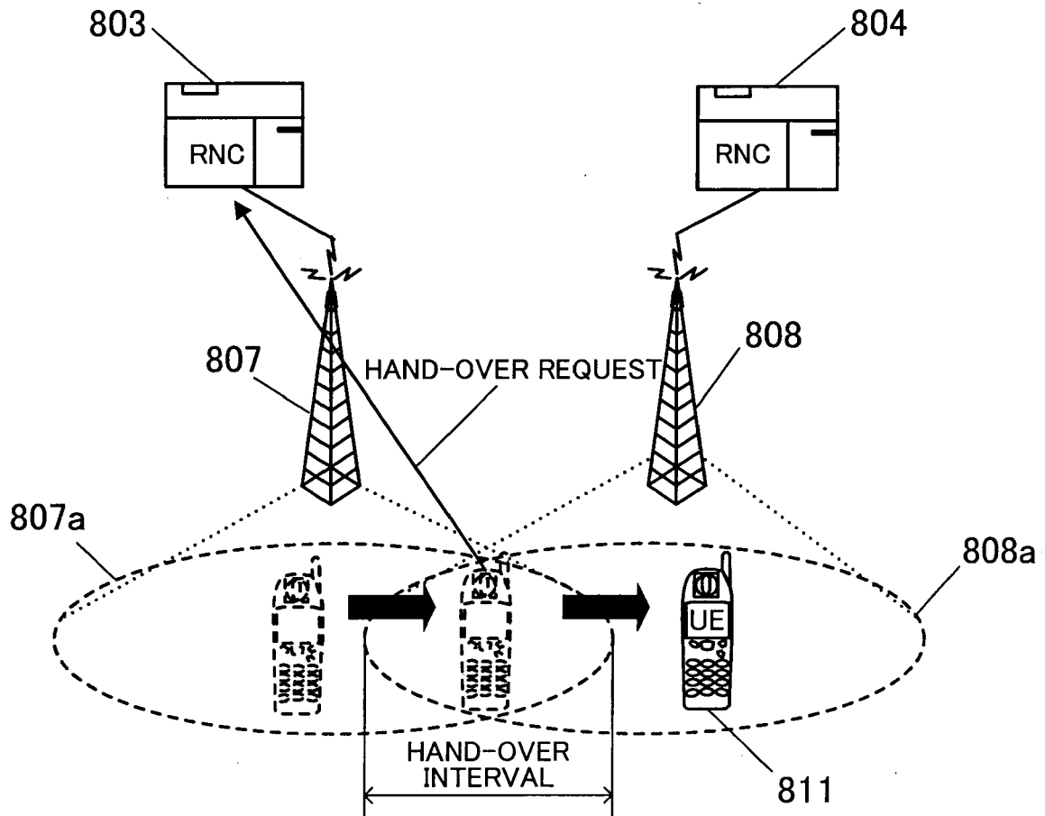
FIG. 24 PRIOR ART
