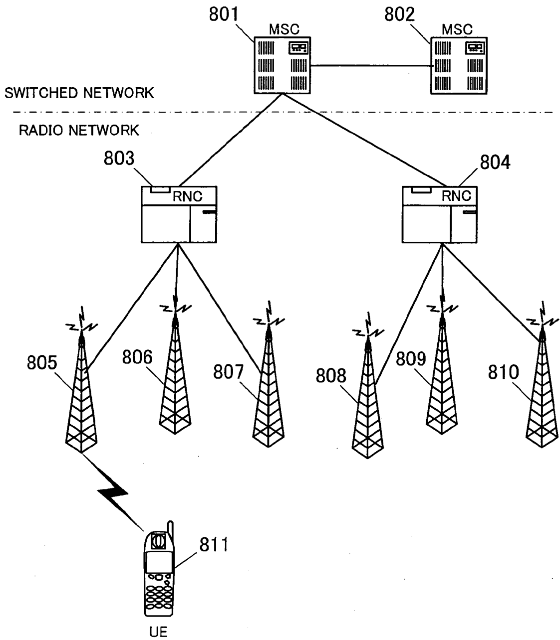
FIG. 23 PRIOR ART
