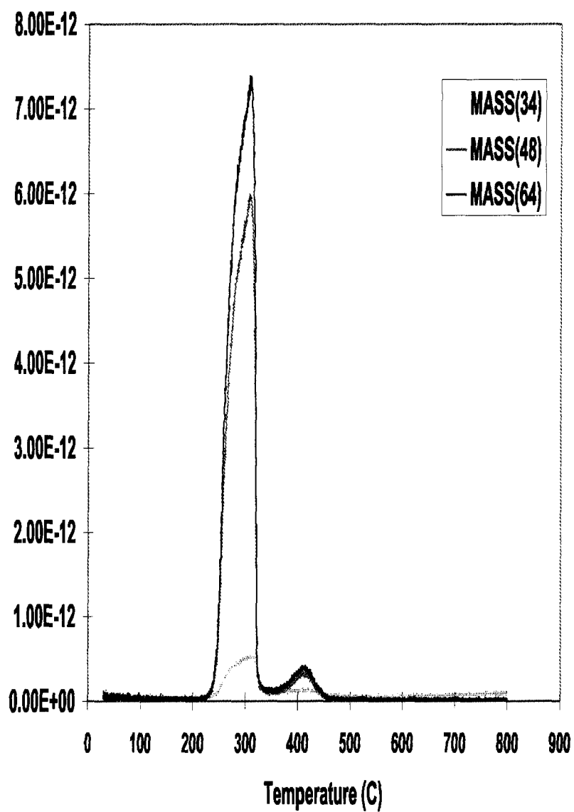
Fig.4. TPR-MS of \text{Cu}_{0.25}\text{SiO}_2(0.75) , sulfated at 500C (ID030)
