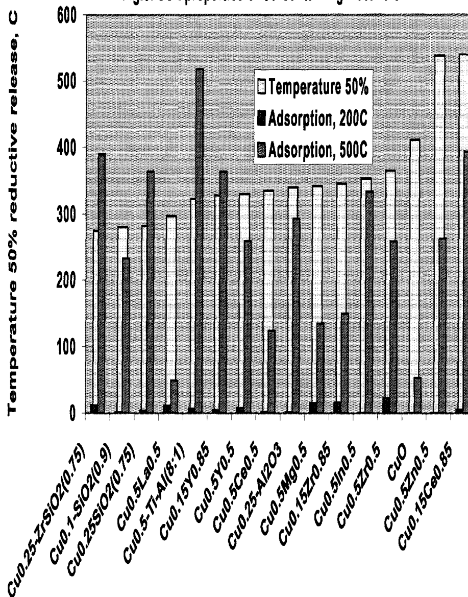
Fig.3. SOx properties of Cu-containing materials
