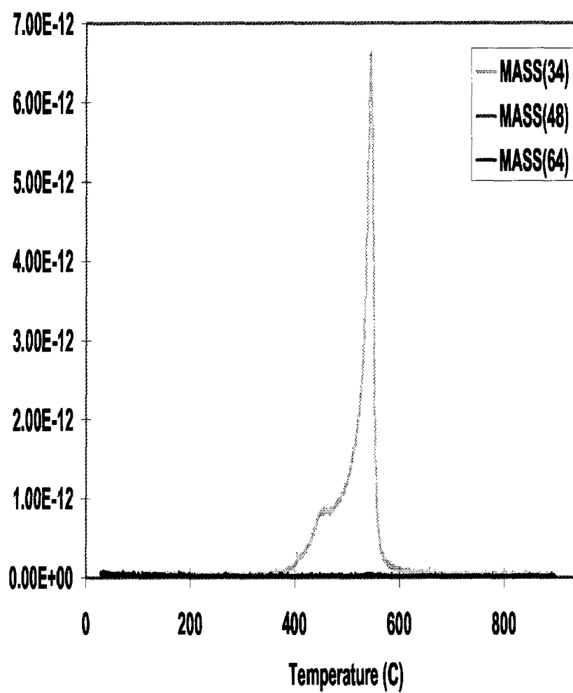
Fig.2.TPR-MS of sulfated Pt-CeZr1:1(#50)
