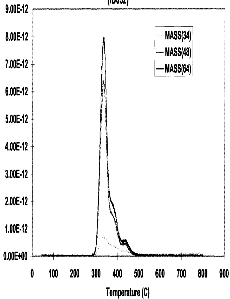
Fig.6. TPR-MS of Cu 0.25 -gamma Al 2 O 3 (0.75), sulfated at 500C (ID032)
