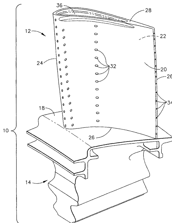
FIG. 1 (PRIOR ART)
