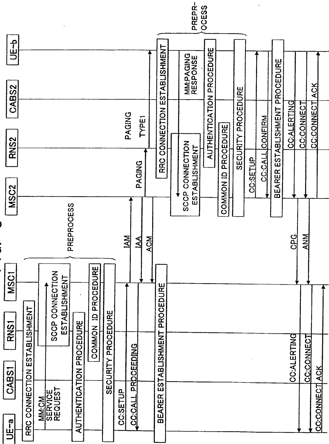
FIG. 8 PRIOR ART
