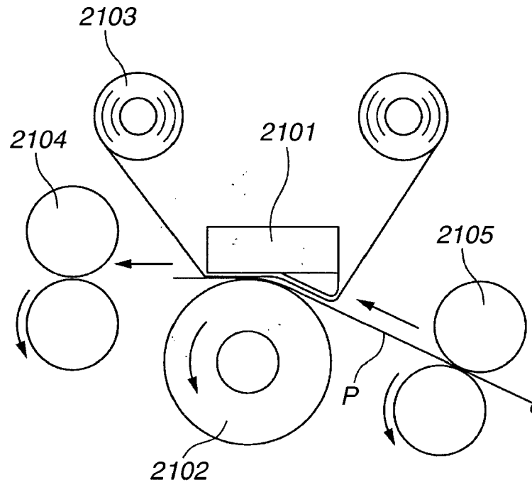
FIG.26 PRIOR ART
