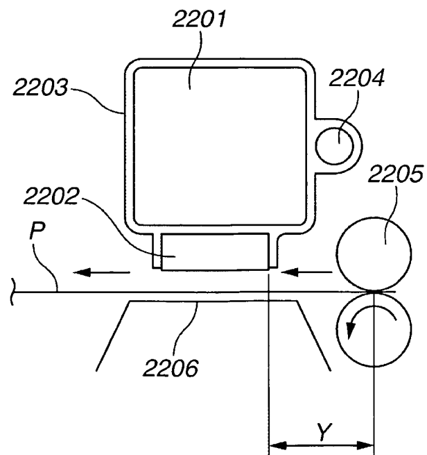
FIG.25 PRIOR ART
