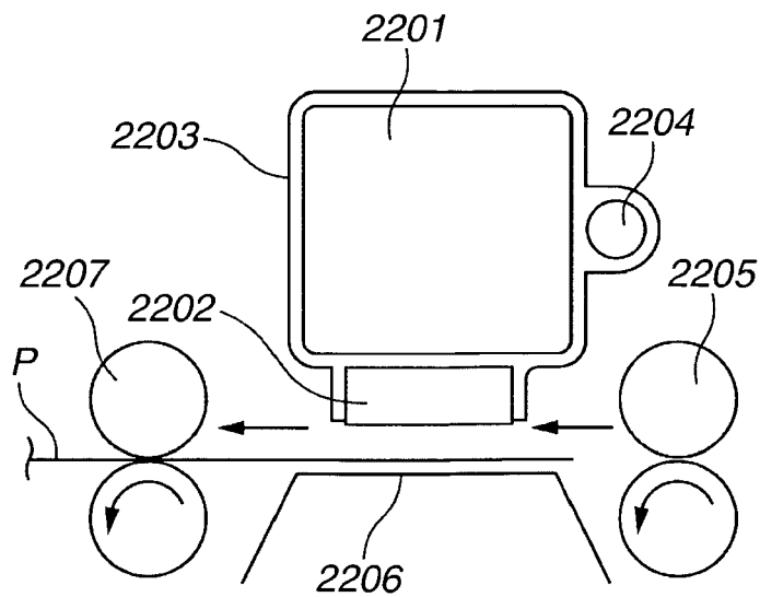
FIG.27 PRIOR ART
