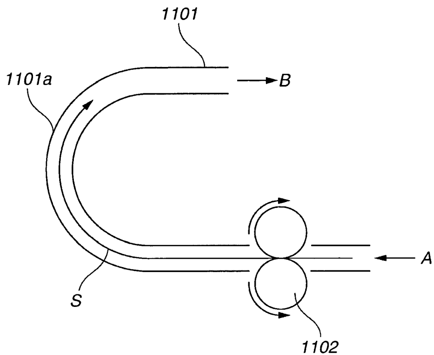
FIG.22 PRIOR ART
