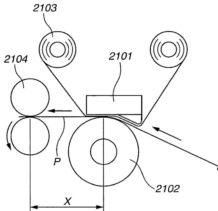
FIG.24 PRIOR ART
