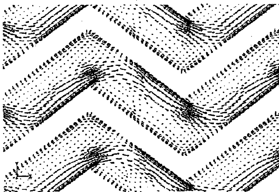
(a) Prior art zigzag flow path
