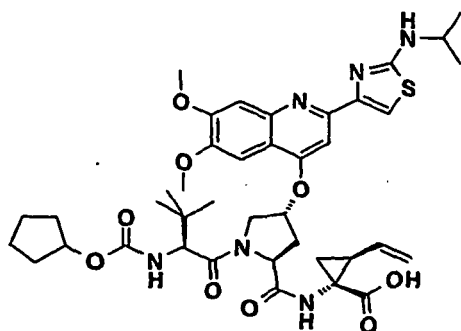
Compound 4014
