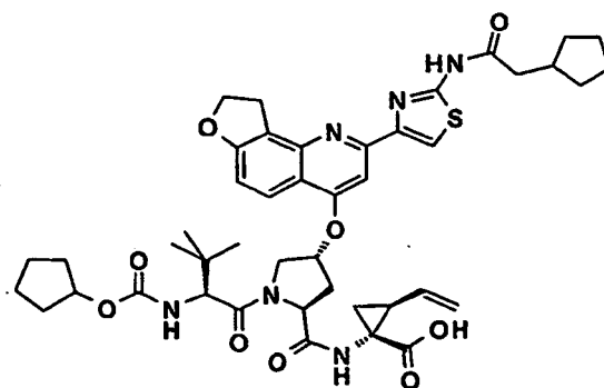
Compound 3010
