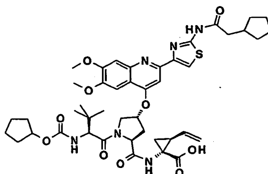
Compound 4013
