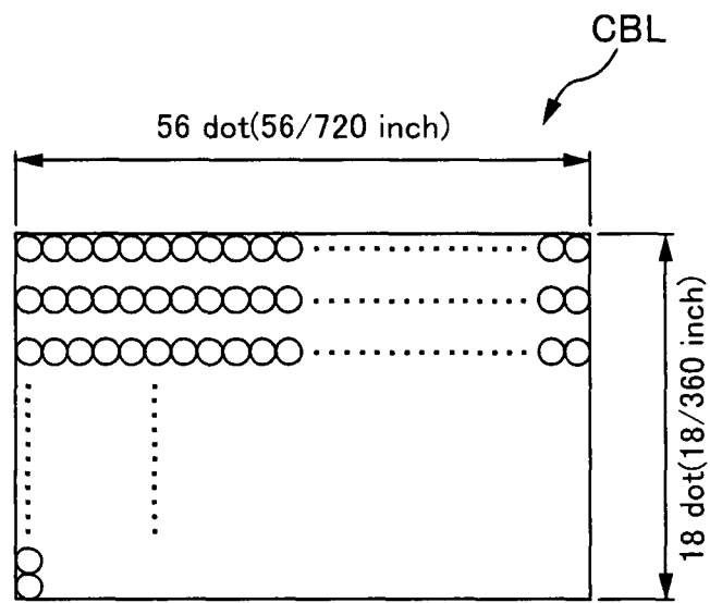
UNIT BLOCK
