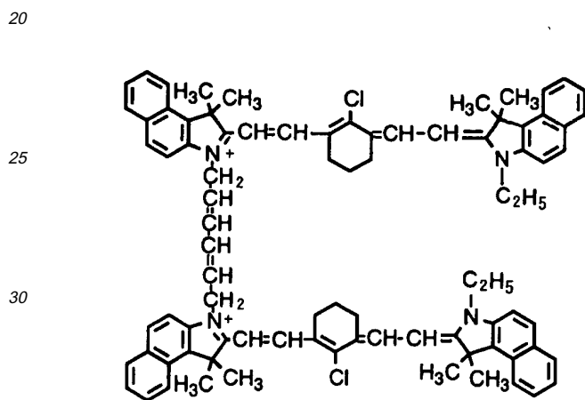
Chemical Formula 6:
