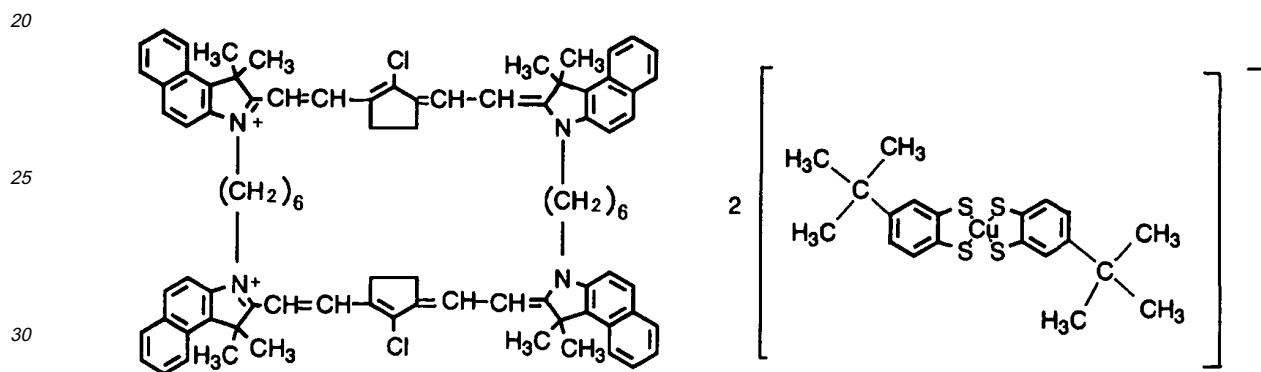
Chemical Formula 12:
