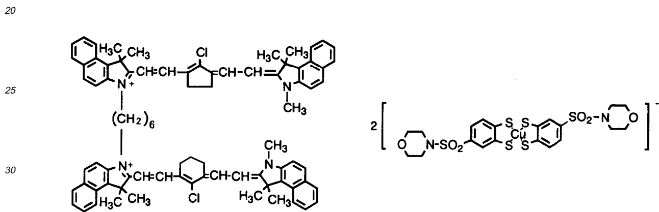
Chemical Formula 18:
