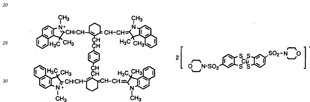
Chemical Formula 21:
