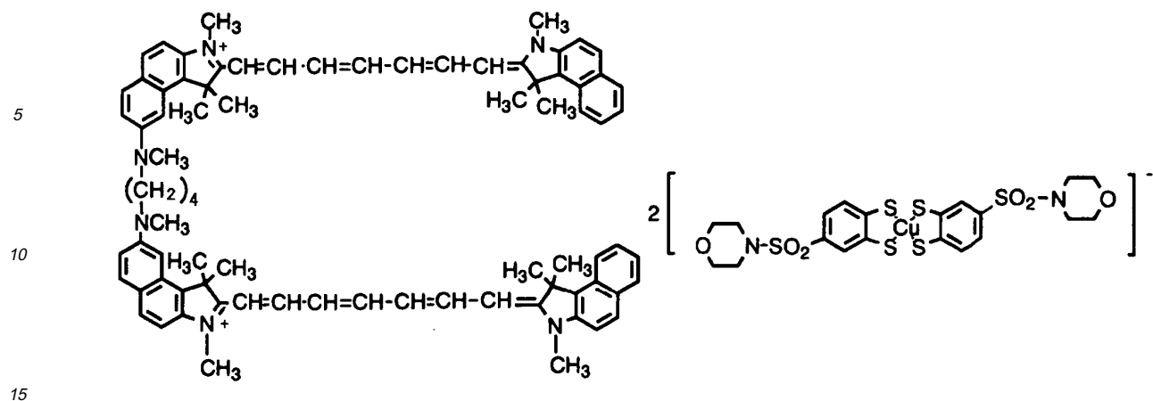
Chemical Formula 18:
