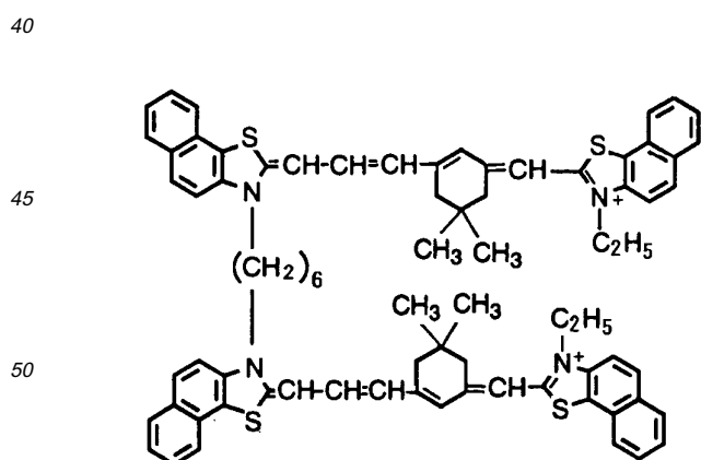
Chemical Formula 7:
