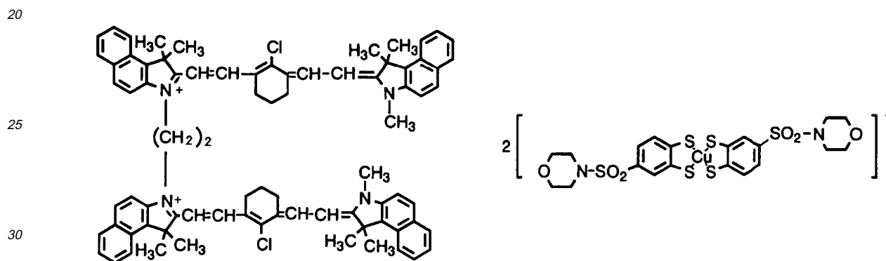
Chemical Formula 9:
