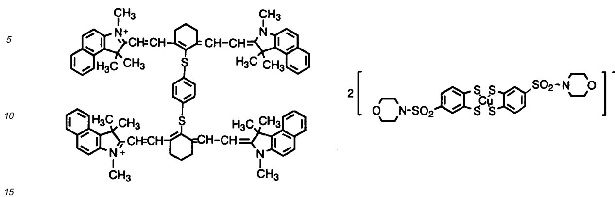
Chemical Formula 21:
