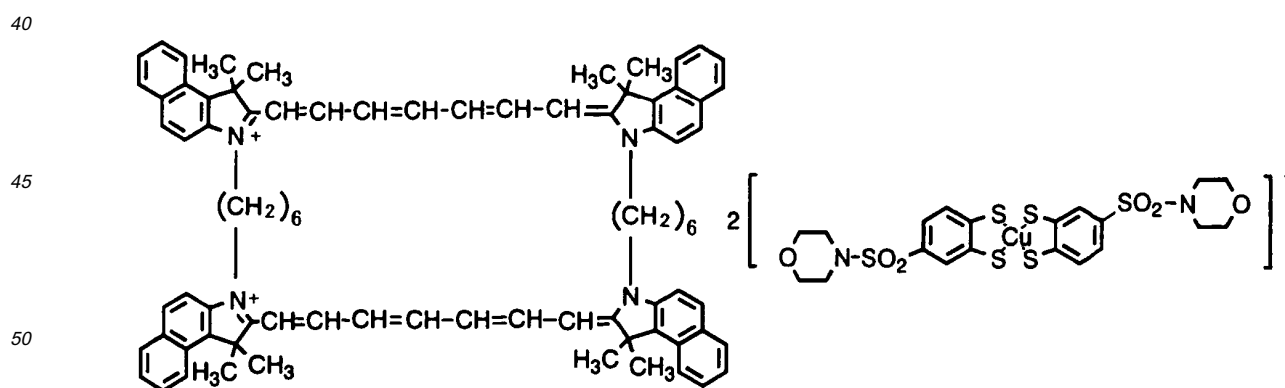
Chemical Formula 11:
