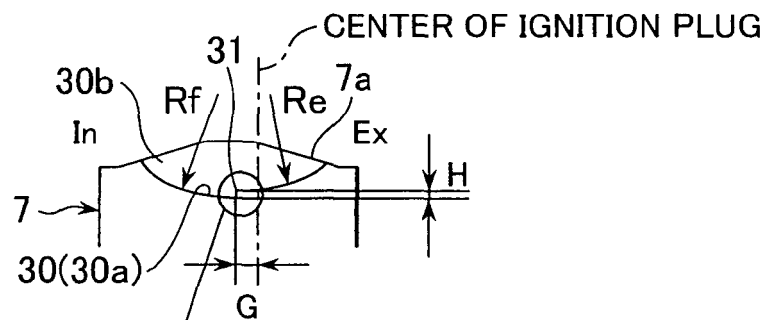
FIG. 4D IN ENLARGED SCALE
