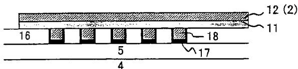
(e) A—A' Cross Sectional View
