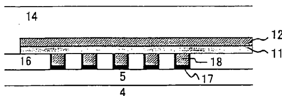
(g) A—A' Cross Sectional View
