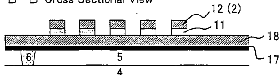
B—B' Cross Sectional View
