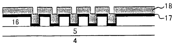
(c) A—A' Cross Sectional View
