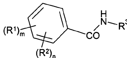
Formula (Ib)
