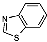
benzothiazole
