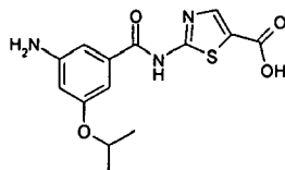
Compound (k)
