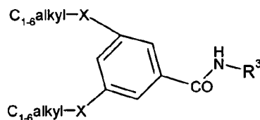
Formula (IId)
