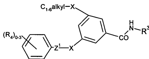
Formula (IIb)
