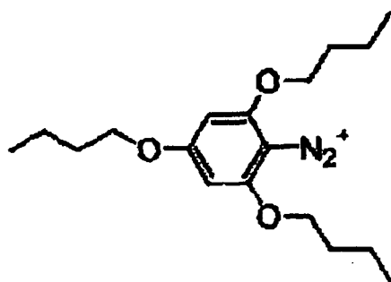
ClO 4 - (N-8)
