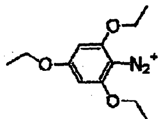
PF 6 - (N-2)
