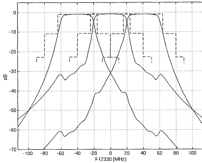
FIG. 12 Selectivity
