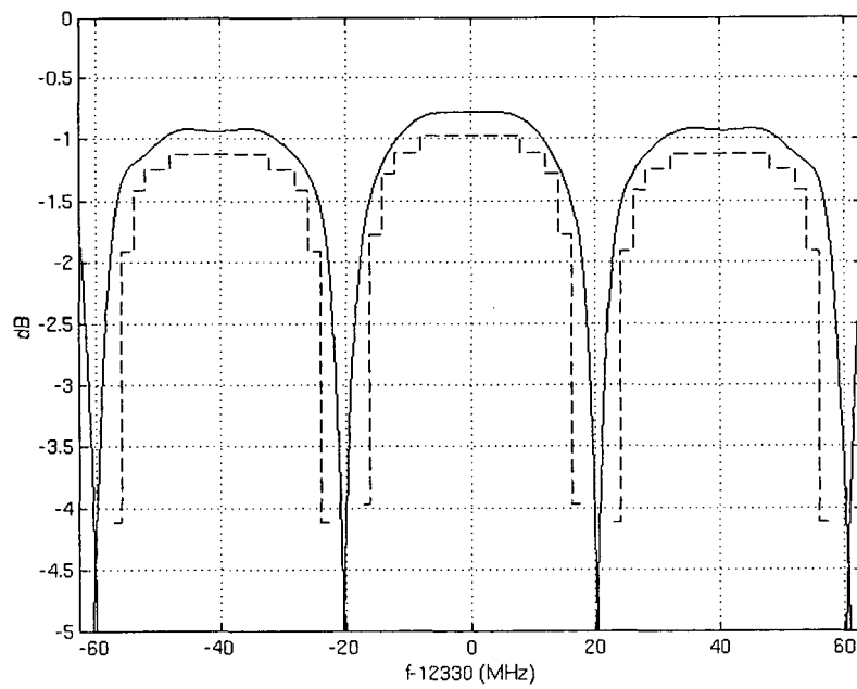
FIG. 13 Insertion Loss Flatness
