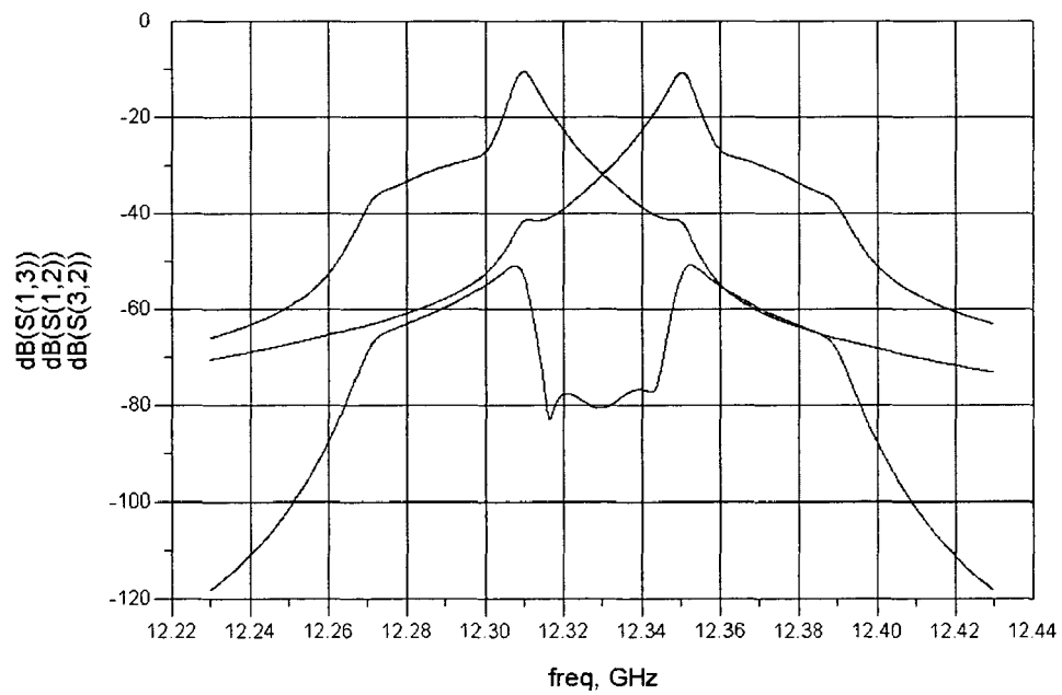
FIG. 17 Isolation between channels
