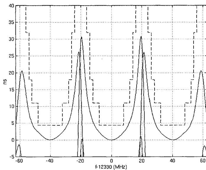
FIG. 14 Channels group delay
