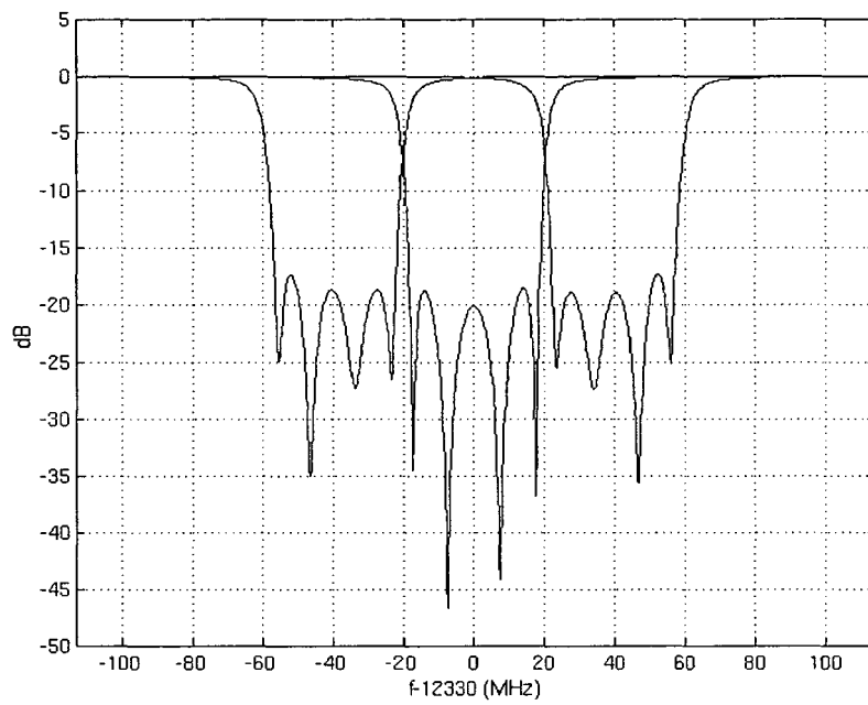
FIG. 16 Channel output port return loss
