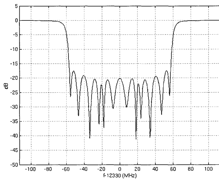
FIG. 15 Common port return loss
