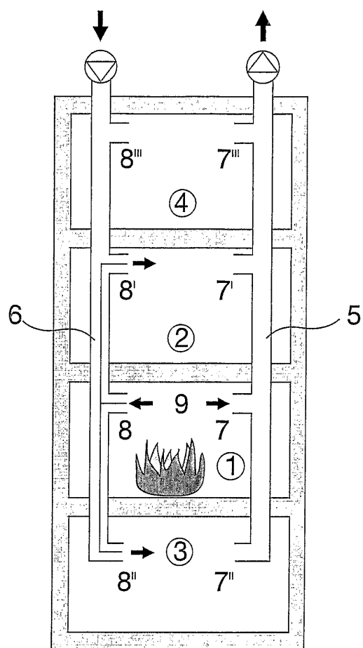
Fig 1 (Prior Art)
