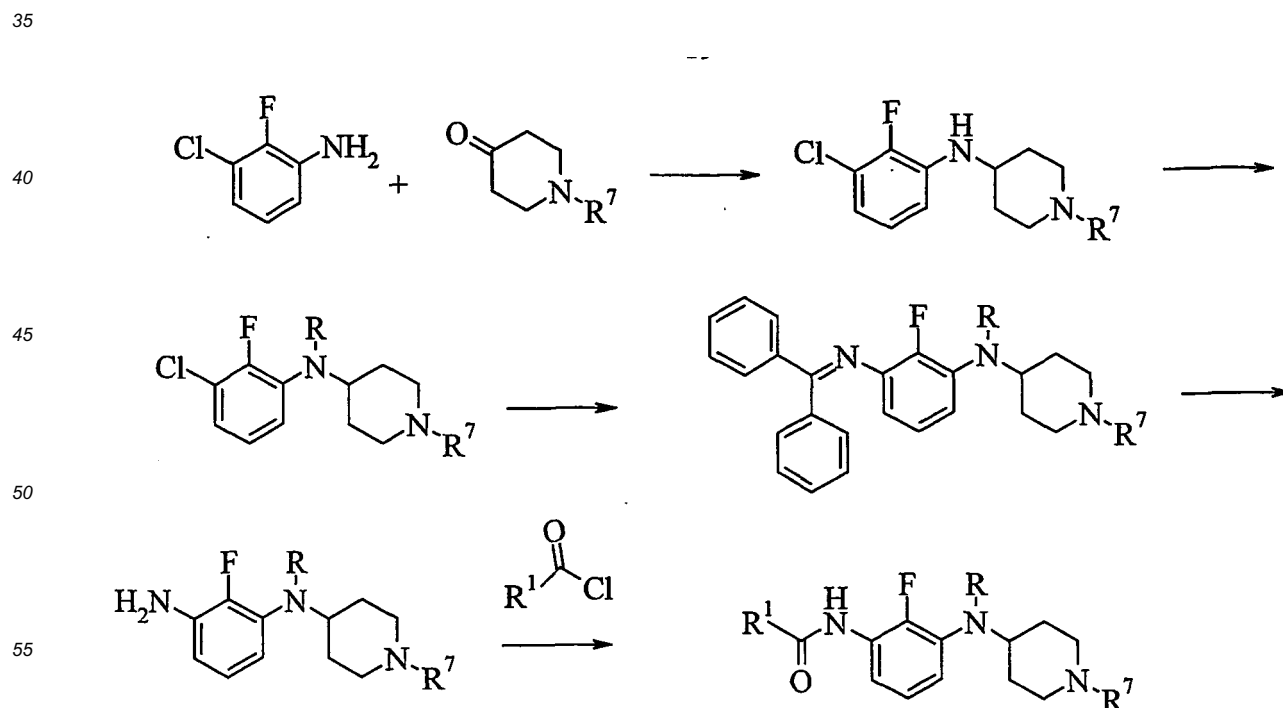
Scheme 4:
