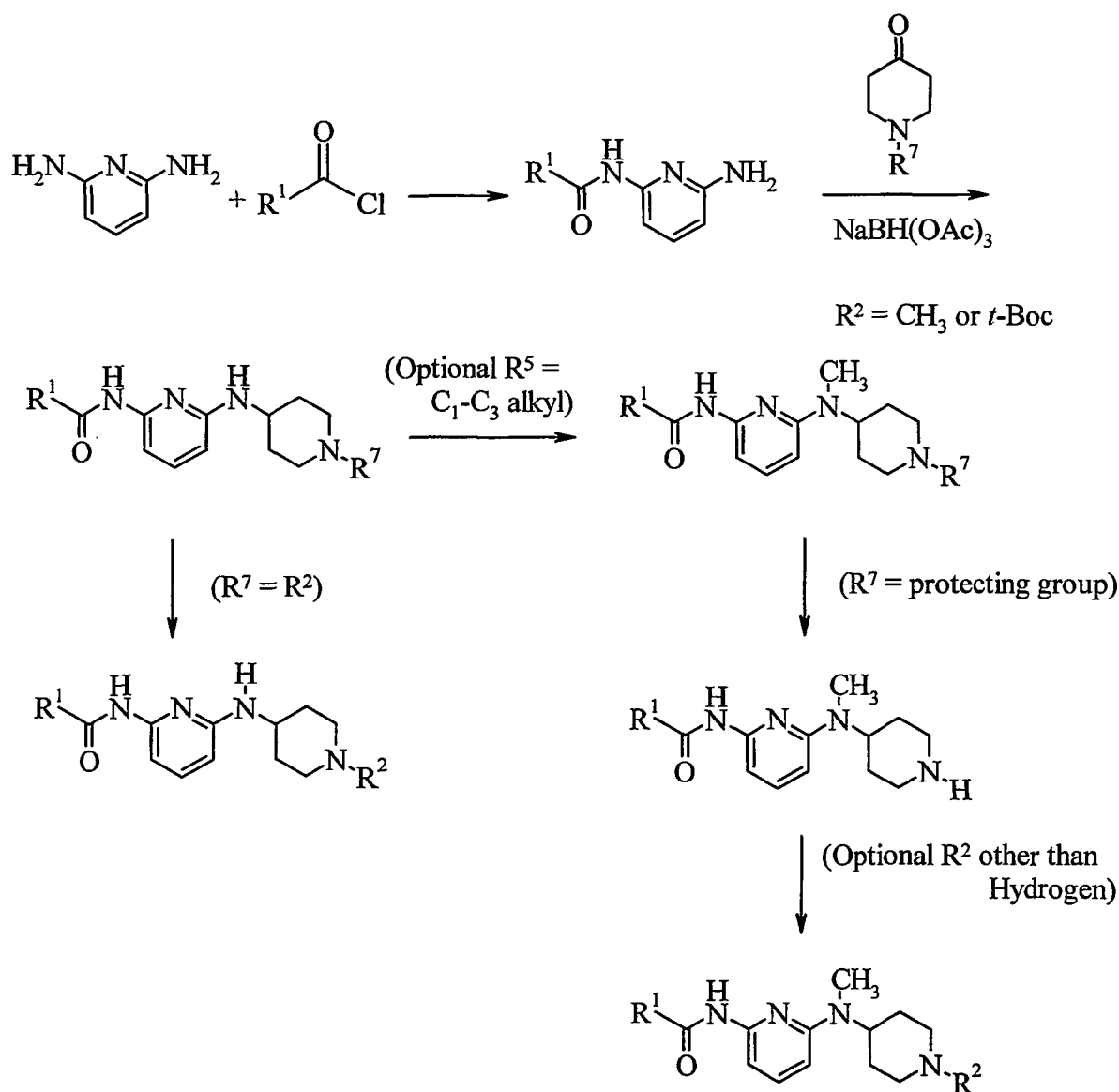
Scheme 9:
