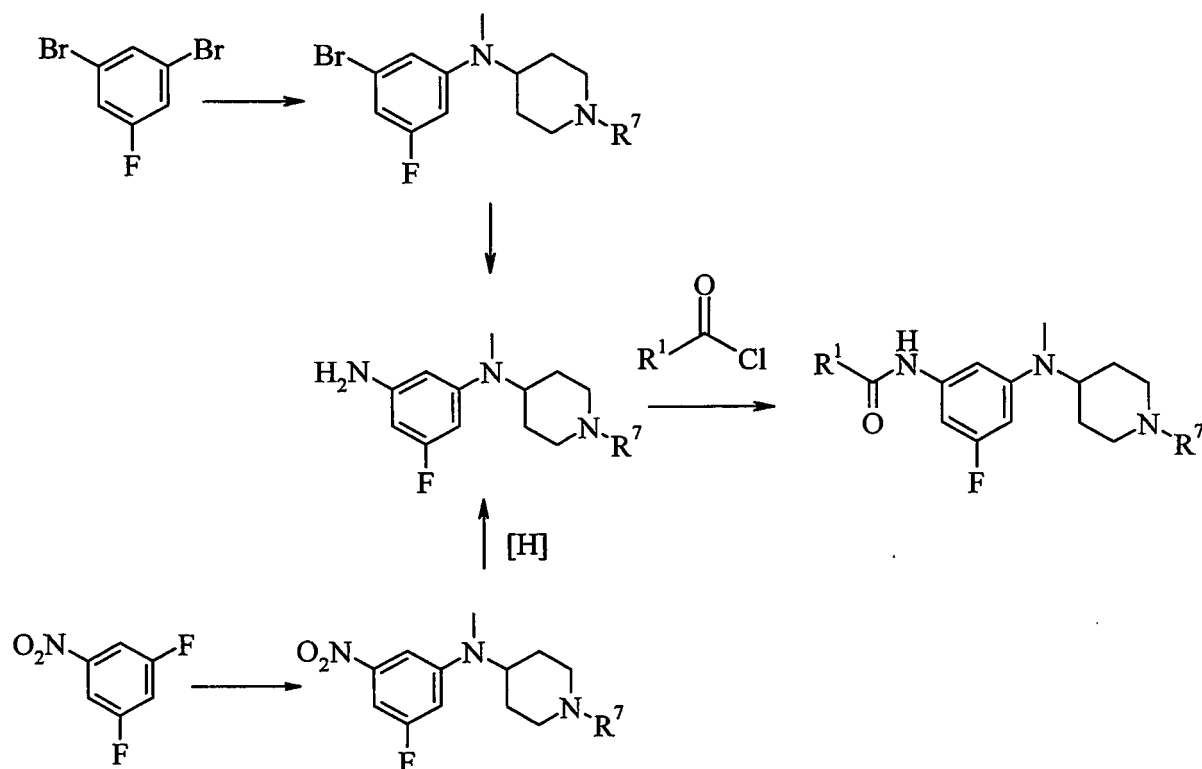
Scheme 6:
