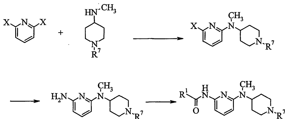
Scheme 8:
