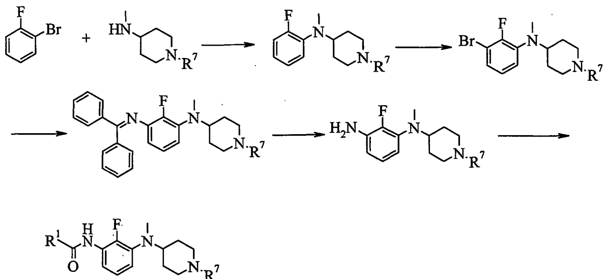
Scheme 5:
