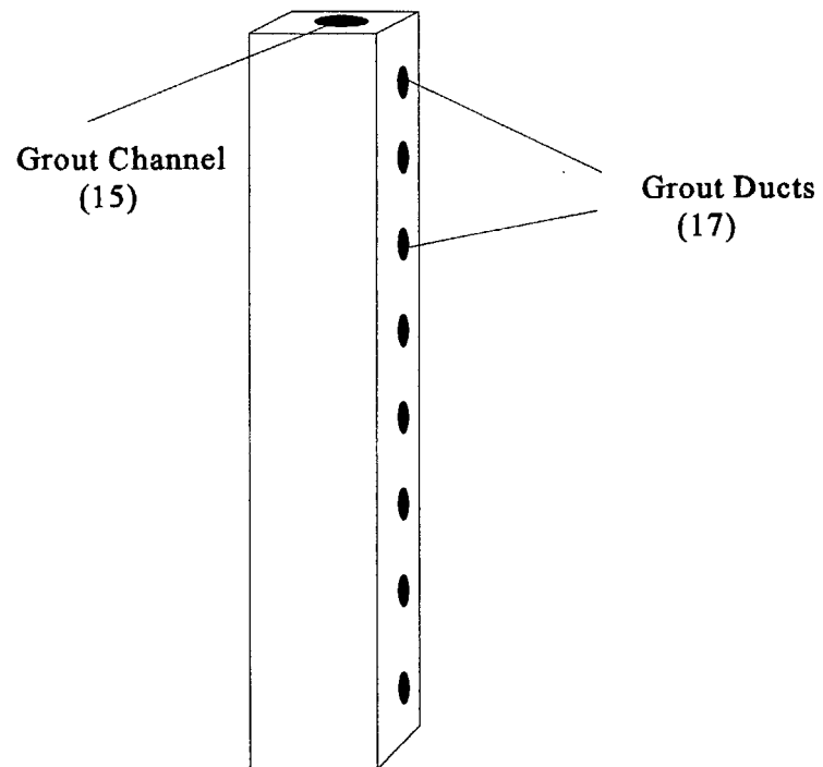
Fig. 6 A - Locking Post (12)
