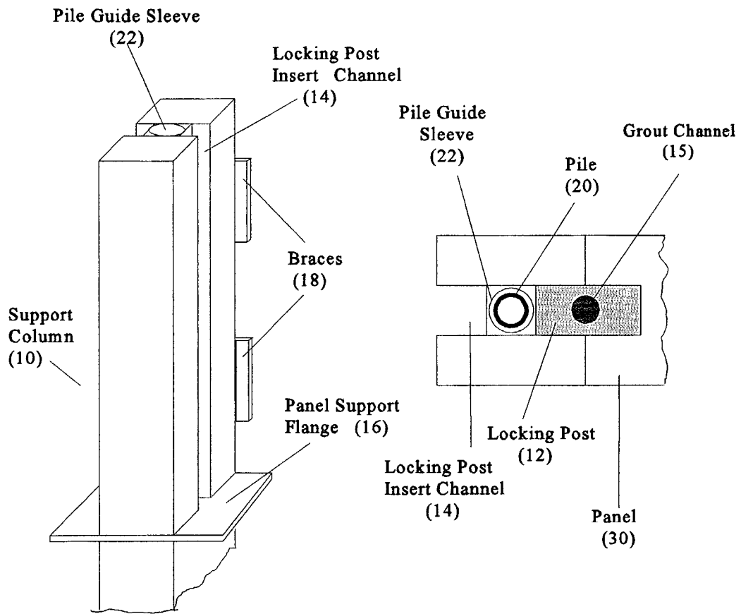
Figure 3B. Support Column Top View
