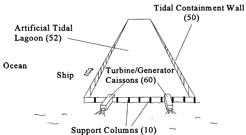
Fig. 1 A - Tidal Energy System (60) : Completely Offshore
