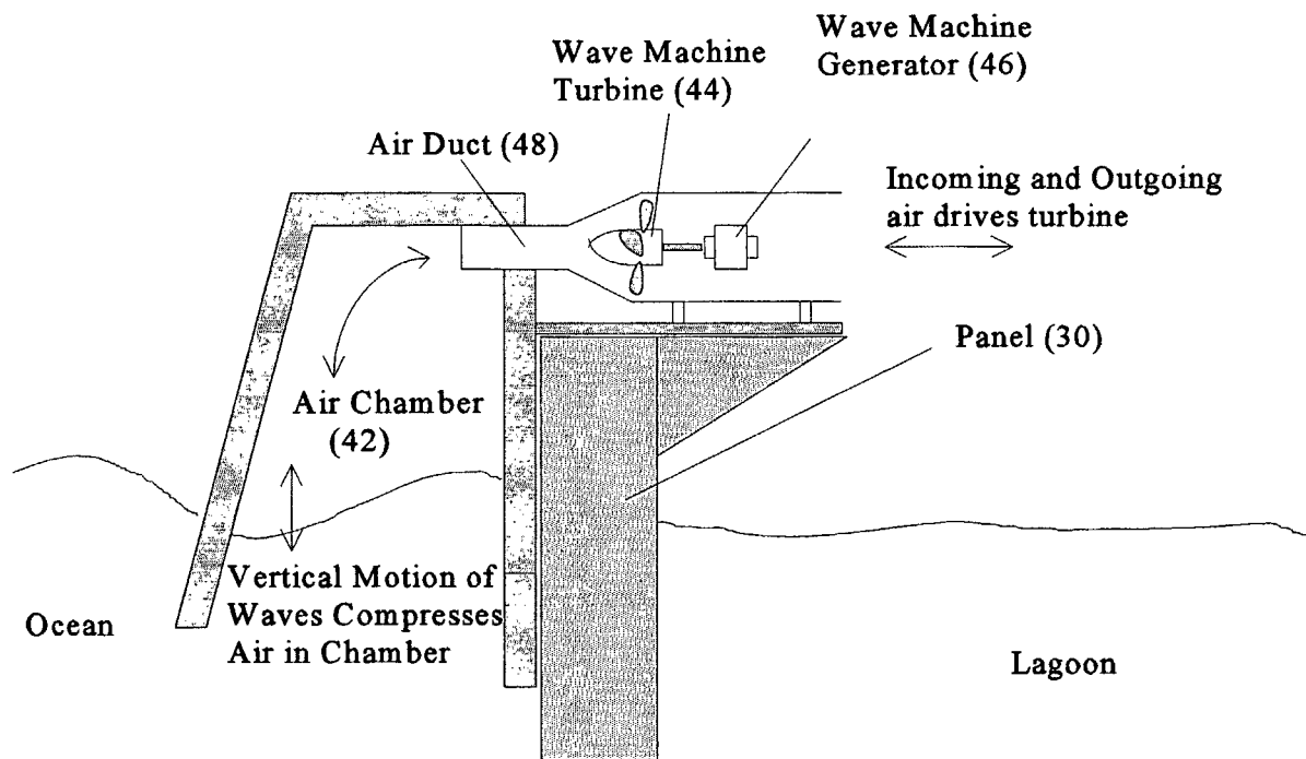
Fig. 8 - Wave Machine (40) Mounted on The Top Panel of a Tidal Containment Wall Section
