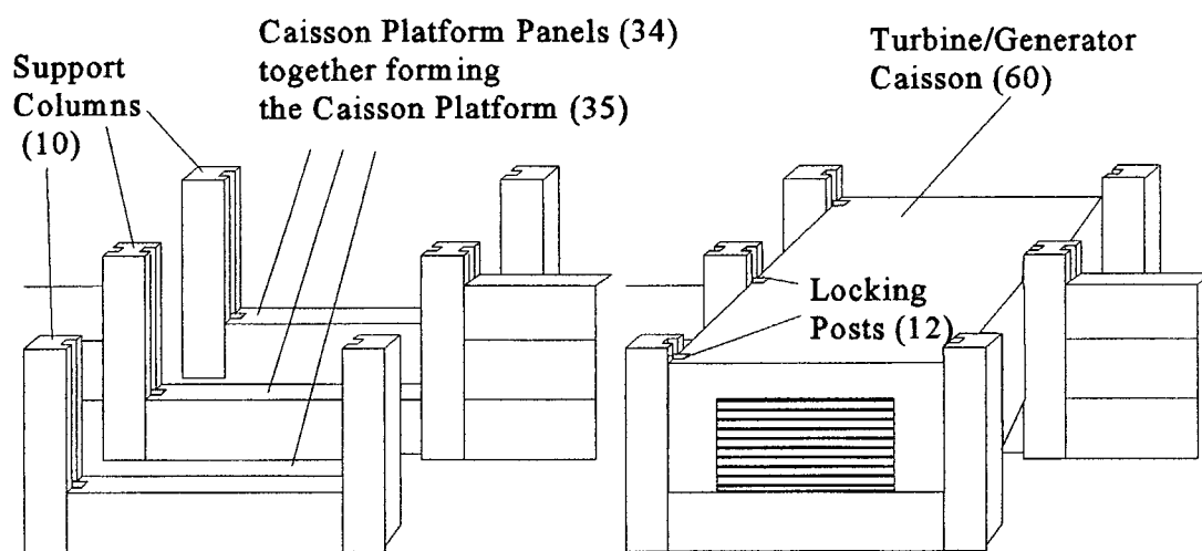
Fig. 7 A. The Caisson Platform
