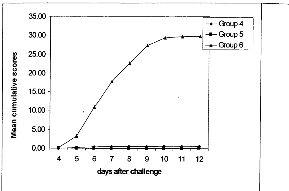
Figure 6, Mean cumulative HSV lesion scores (see example 3)
