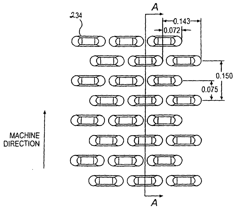
FIGURE 18B
