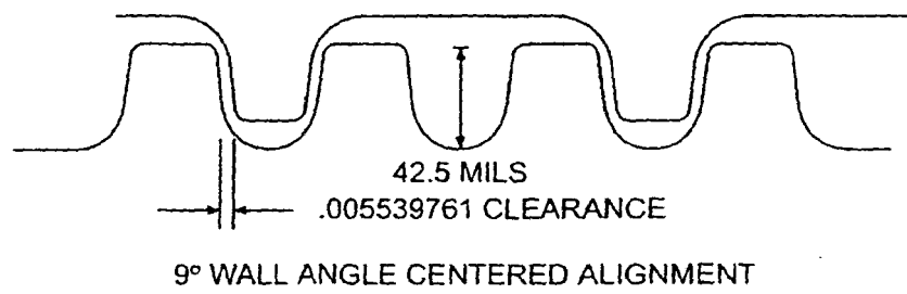
FIGURE 22B
