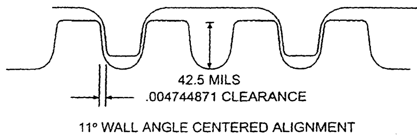
FIGURE 22C
