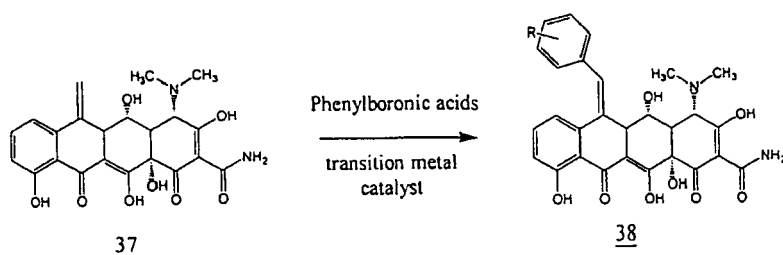
Scheme XI
