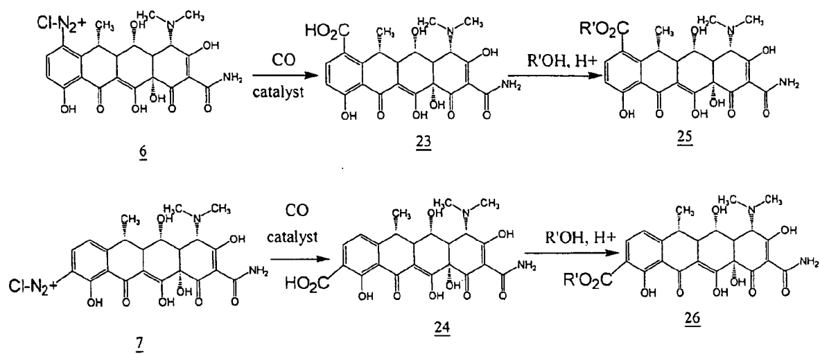
Scheme IX
