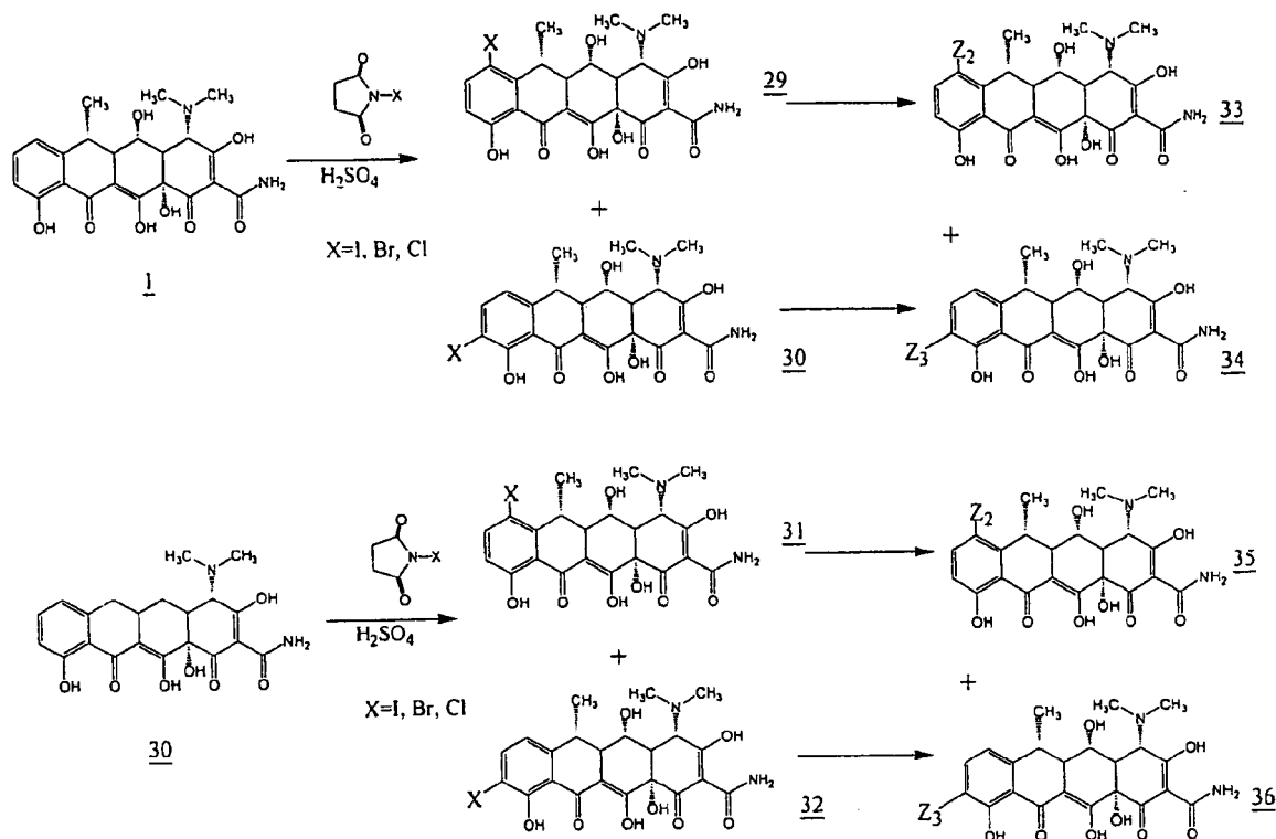
Scheme X
