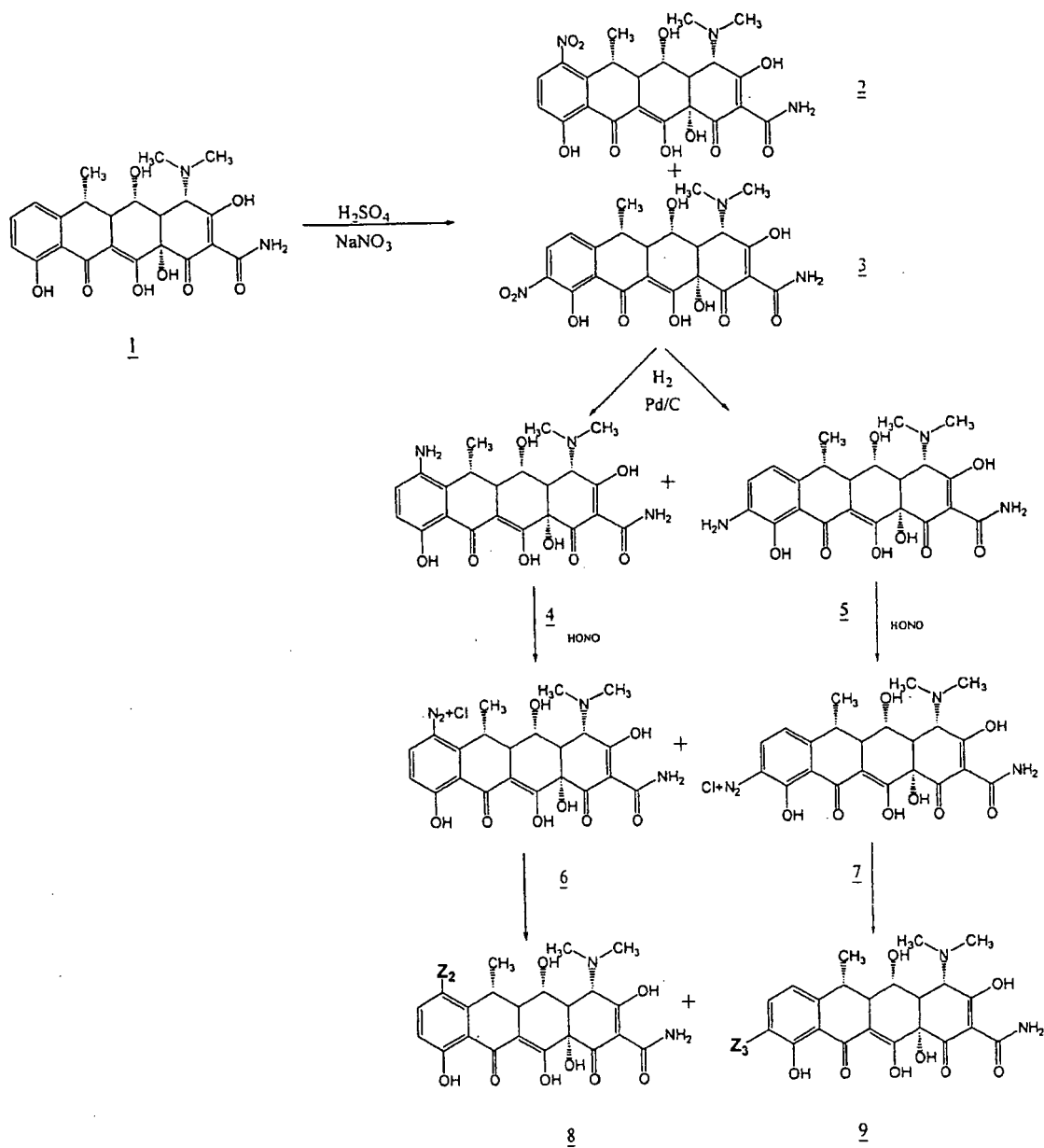
Scheme 1
