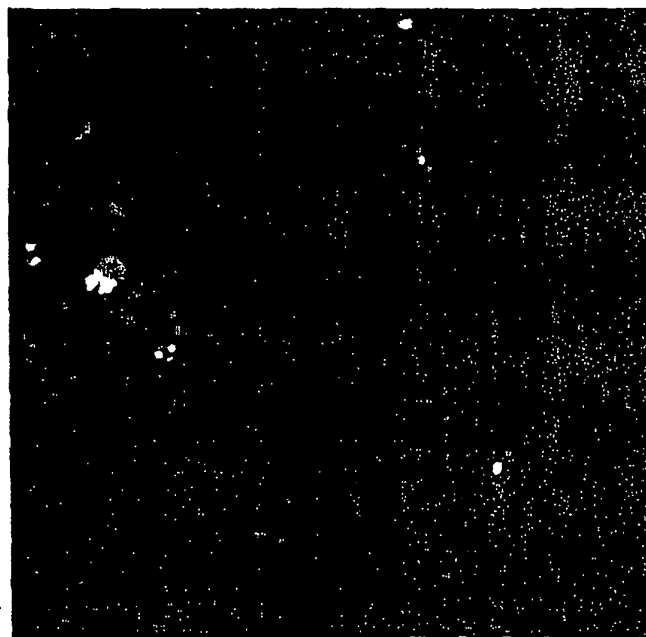
686 Alloy - Exposed to \text{LiBF}_4/\text{GBL} during Cyclic Polarization test - 5000X
