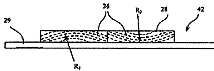
FIG. 8B (cross-section)
