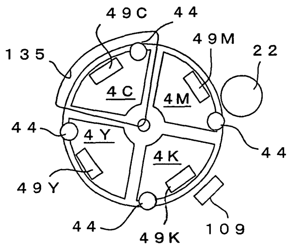
FIG. 5C : MOUNTING/DISMOUNTING POSITION
