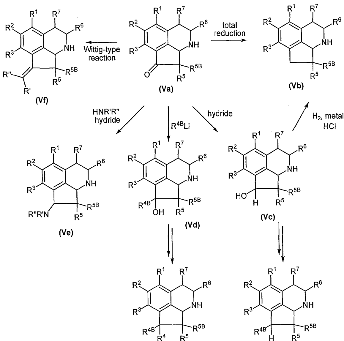
Scheme 7
