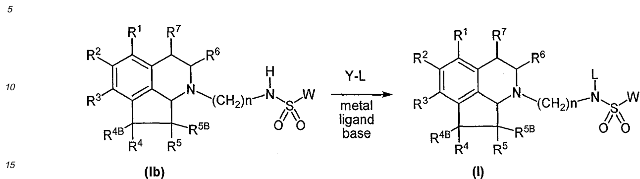
Scheme 14
