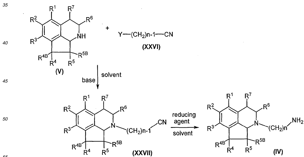
Scheme 19
