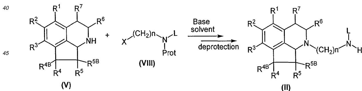
Scheme 5
