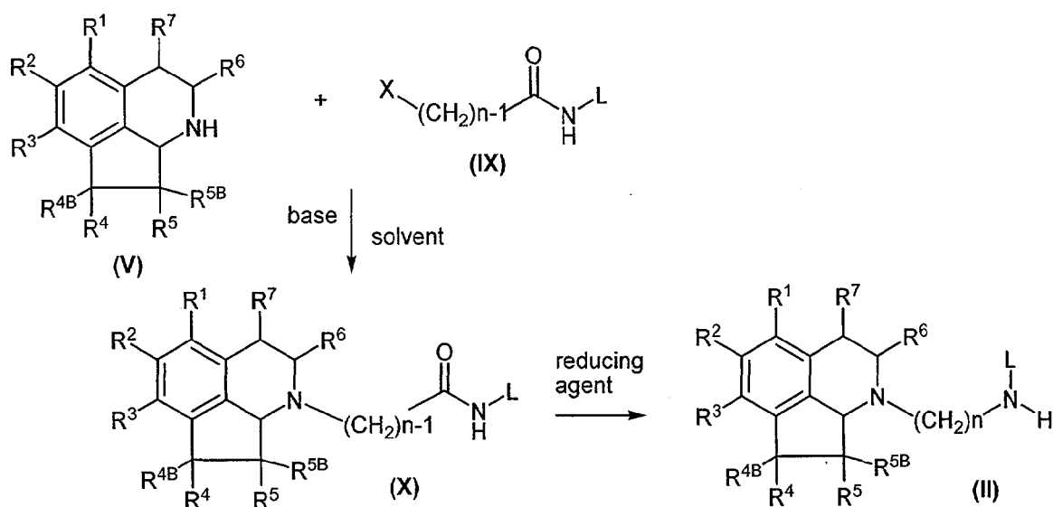
Scheme 6
