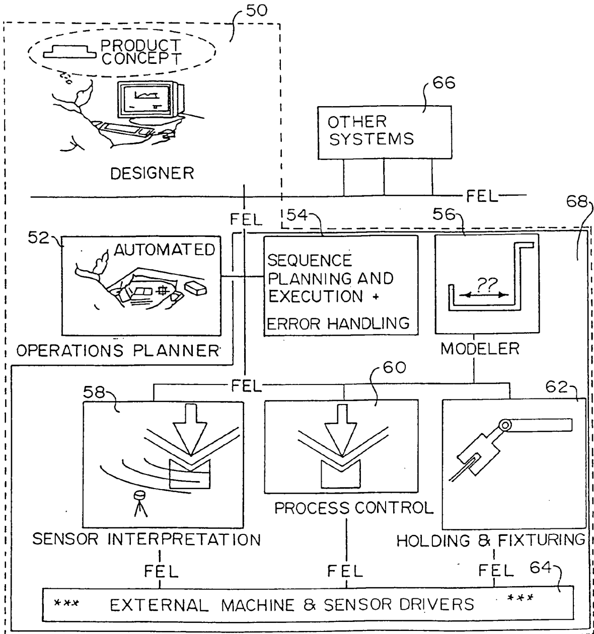
FIG. 4 PRIOR ART
