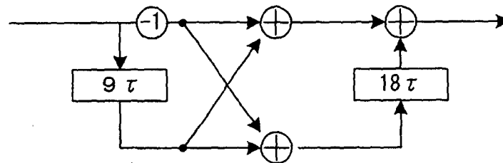
FIG. 12B B MATCHED FILTER
