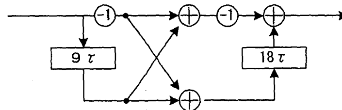
FIG. 12D D MATCHED FILTER
