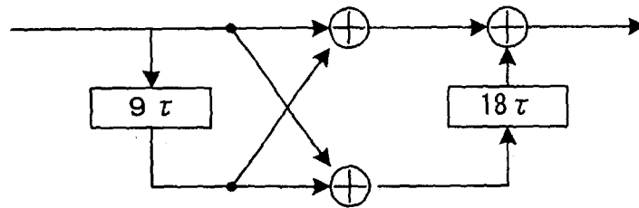
FIG. 12A A MATCHED FILTER
