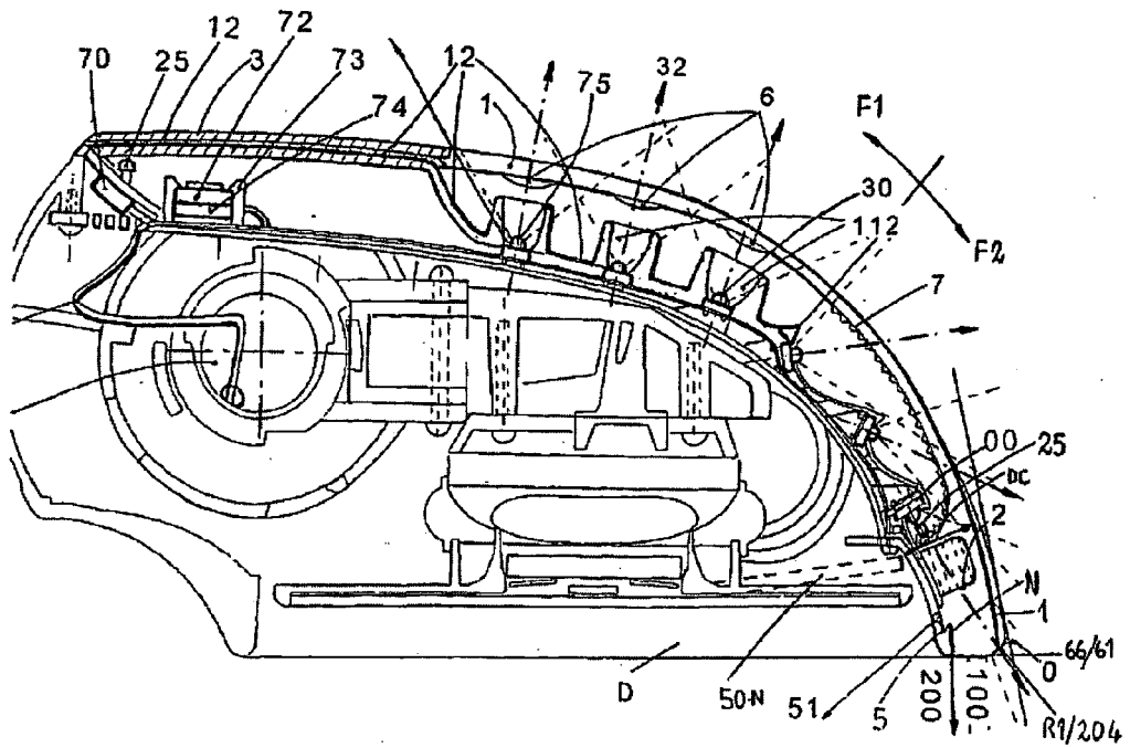
FIG.52 SECTION B-B
