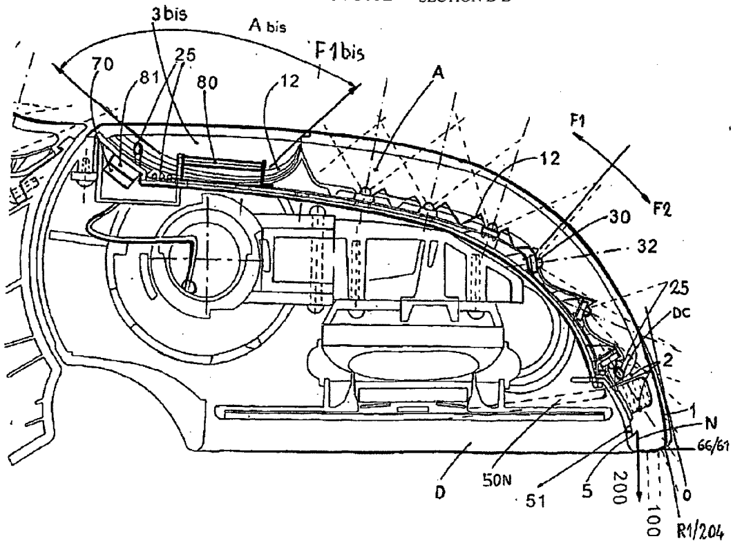
FIG.52 SECTION B-B
