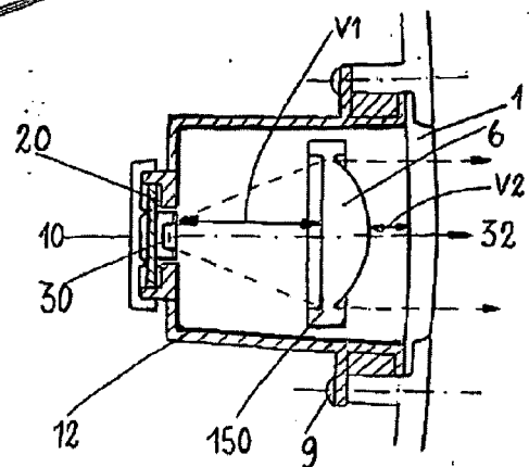
FIG.67 SECTION A-A
