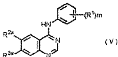
[Chem. 17]
