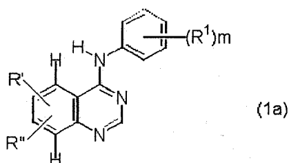
[Chem. 1]
